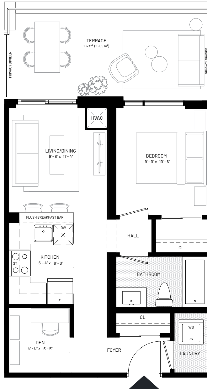
LEVEL 3
